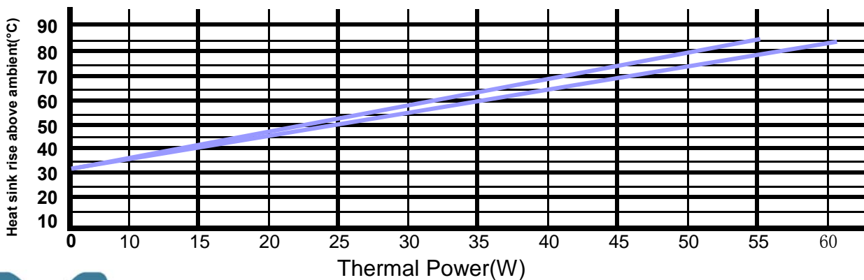
Heat sink to ambient temperature rise T_{hs-amb}(^{\circ}C)
